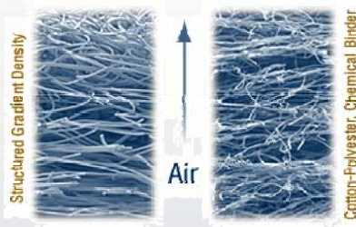
Figure 1: INTREPID® Filtration Media (Charged-Mechanical)
