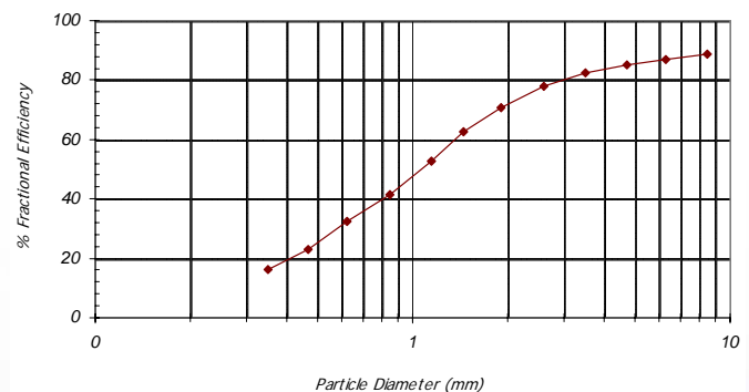
Efficiency vs. Particle Diameter
